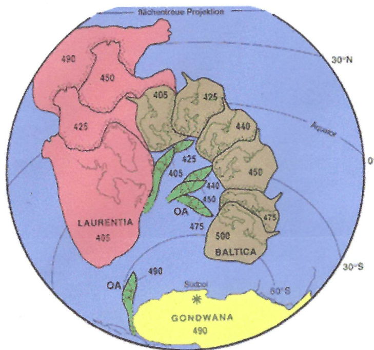
One concept of Baltican evolution in the early Paleozoic
